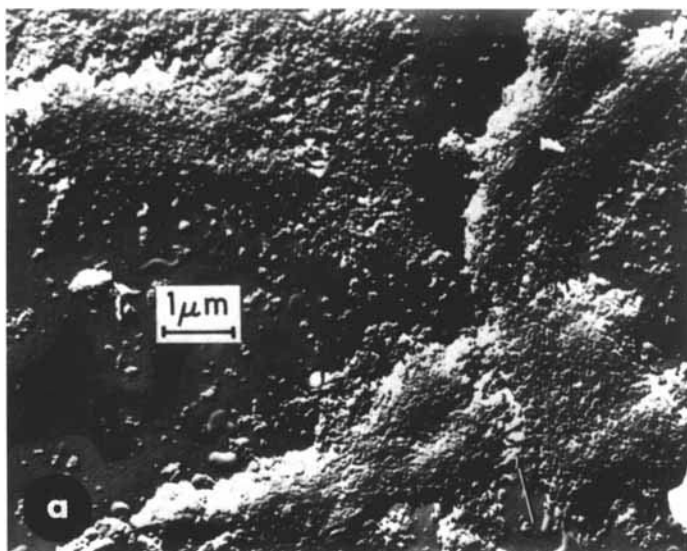
Fig. 5. S:O (Pt-C shadowed, 35°) replicas of wet unstained and unfixed Chinese hamster chromosomes in a metaphase spread.
